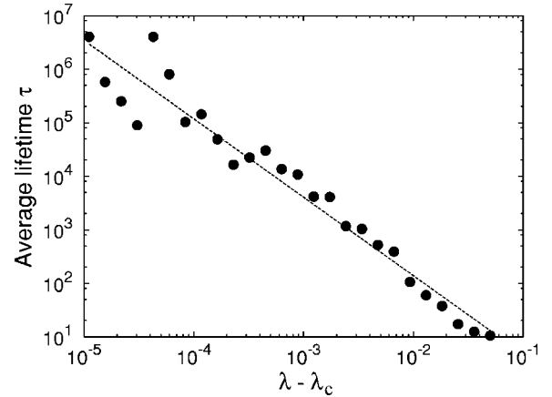
FIG. 13. Dependence of the average lifetime on the parameter \lambda . The linear fitting indicated by the dashed line yields a critical exponent \gamma \approx 1.46 in Eq. (16).
