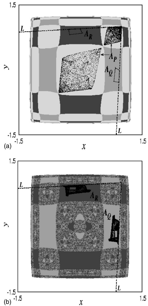
FIG. 8. Basin structures before and after the boundary crisis: (a) total basins of A_P (silver), A_Q (light gray) and A_R (dark gray) where (\lambda, \epsilon)=(1.53, 1.9) ; (b) fractal basin boundary separating the total basins of A_Q (light gray) and A_R (dark gray) where (\lambda, \epsilon)=(1.62, 1.9) .
